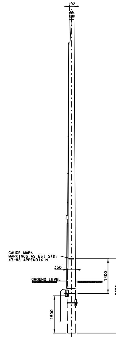
TRANSVERSE ELEVATION
