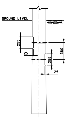
DIMENSIONS FOR NOTCHINGS (SCALE 1:25)
